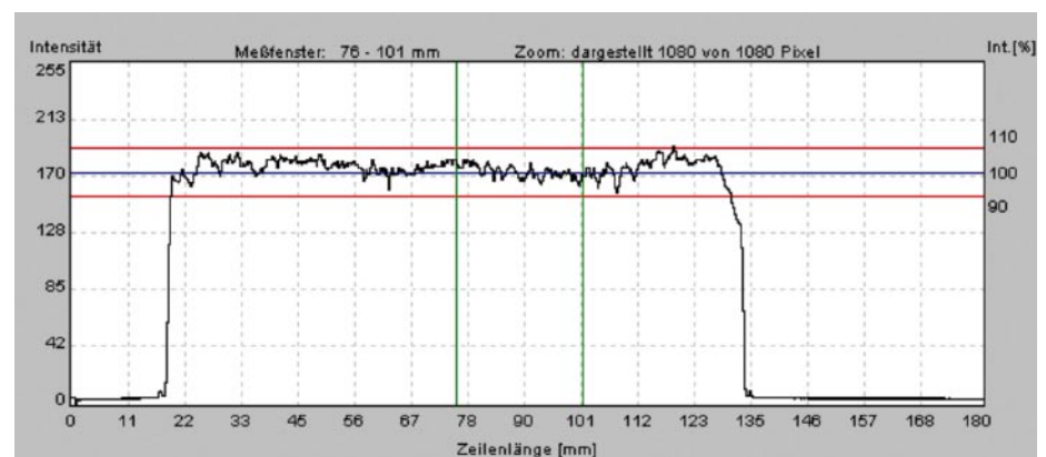
Dragonline shows very good light uniformity values of +/- 10% over the whole line length. A cos4-effect falloff at the edges will be corrected by light distribution.
